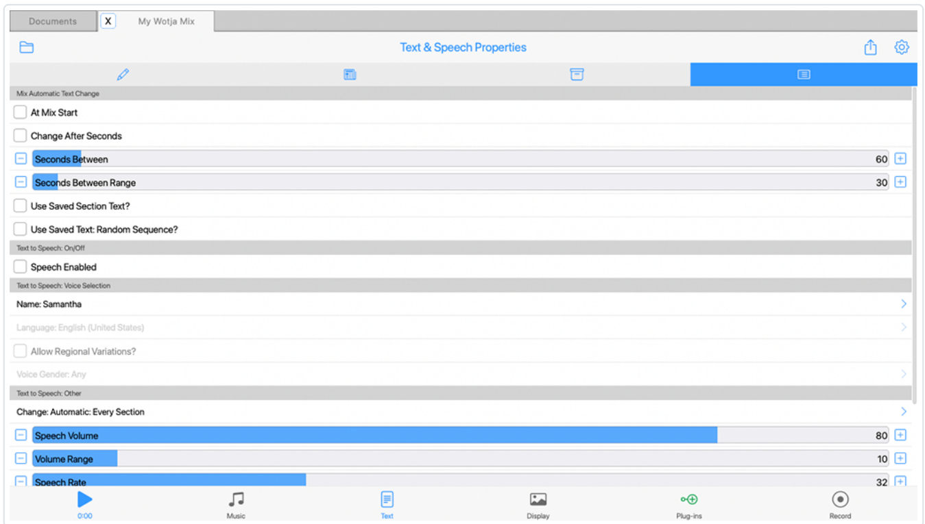
Text Mode: Text Properties Screen
