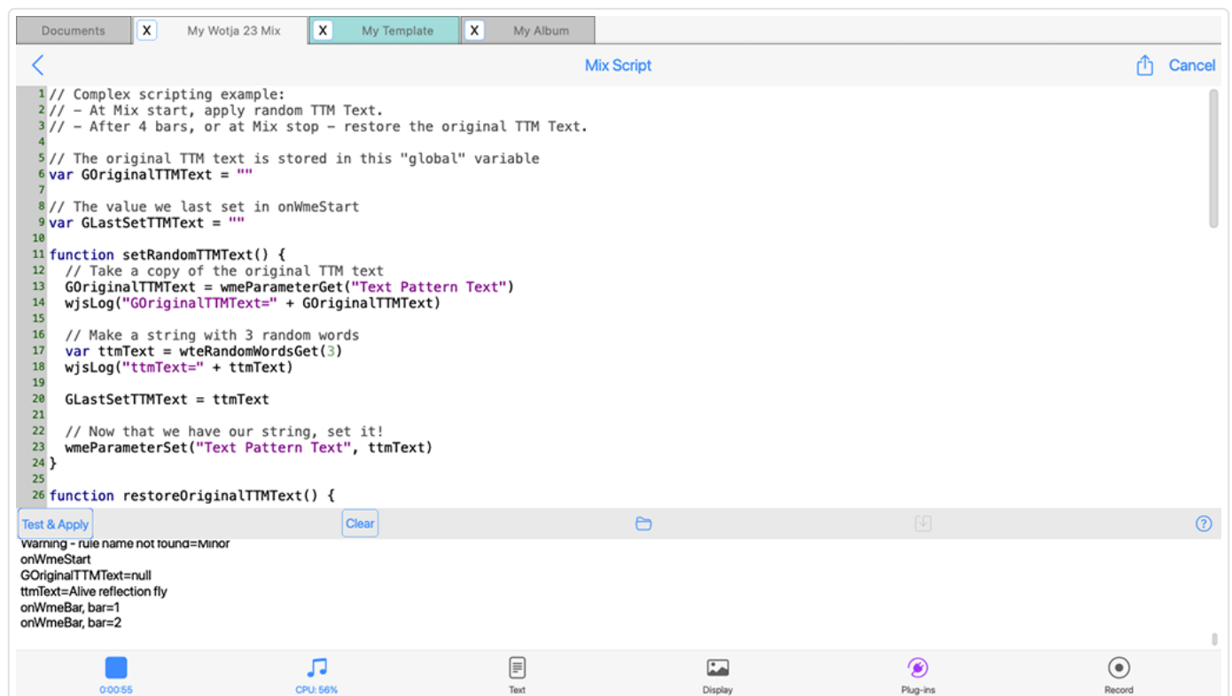
Wotja Script Editor Interface
